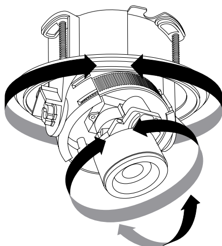
3-achsiger GyroView
